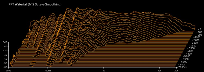
Figure 1. Vicoustic Lab without any acoustic treatment
