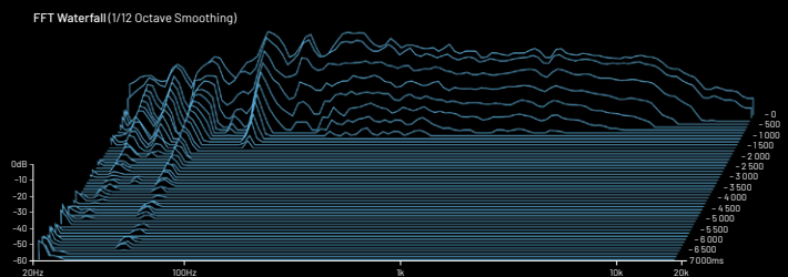
Figure 2. Vicoustic Lab with 4 Mega Bass Trap VMT XXL units
