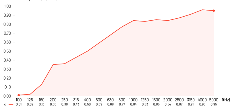
Sound Absorption Coefficient
